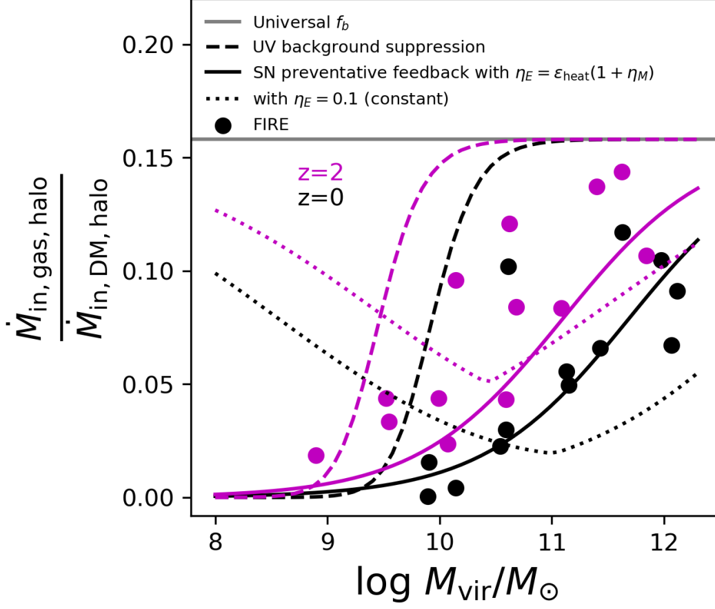
Figure 14. The halo gas accretion efficiency ( \dot{M}_{\text{in,gas}}/\dot{M}_{\text{in,DM}} in the virial shell) as a function of the halo virial mass for the FIRE-2 simulations at z = 0 (black points) and z = 2 (magenta points). If gas accretion perfectly tracked DM accretion at R_{\text{vir}} with the universal baryon fraction ( f_b = 0.158 from Planck Collaboration et al. 2016) as commonly assumed, then the halos would all lie along the horizontal solid gray line. The Okamoto et al. (2008) model describing the suppression of halo gas accretion due to the ionizing UV background is shown with the black dashed line for z = 0 and the magenta dashed line for z = 2 . The FIRE-2 halo gas accretion efficiencies fall below the expectation from UV background heating alone. The dotted lines show the behavior of our simple preventative stellar feedback model if we assume the halo energy loading factor is a constant 0.1; we see that it is incapable of explaining the data points, in fact showing the opposite trend at low masses. However, the solid lines show that our model can explain the data points remarkably well if we assume that the halo energy loading factor is preferentially higher for dwarfs ( \eta_E = \epsilon_{\text{heat}}\eta_M with \epsilon_{\text{heat}} = 0.01 , implying that \eta_E is of order unity for low-mass dwarfs). The agreement is better at z = 0 than z = 2 , suggesting either a redshift dependence for \epsilon_{\text{heat}} or that our simple model is breaking down.
