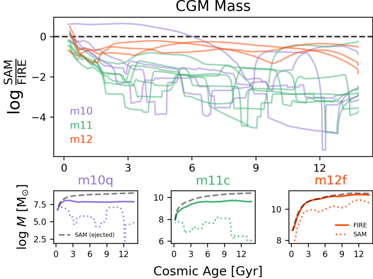
Figure 6. Similar to Figure 3 but now for CGM mass. The SAM predicts much lower CGM masses than FIRE-2 for all halos, with the deficit being worse for the m10 and m11 halos ( \sim 3 - 4 orders of magnitude). In the individual example halo panels (bottom), we overplot the mass of the “ejected gas” reservoir (dashed gray lines) and see that it alone is larger than the FIRE-2 CGM mass. The SAM CGM masses are likely very low because most of the gas resides in this ejected reservoir (i.e., the SAM predicts that most of the extragalactic yet bound gas resides outside of the halo).
