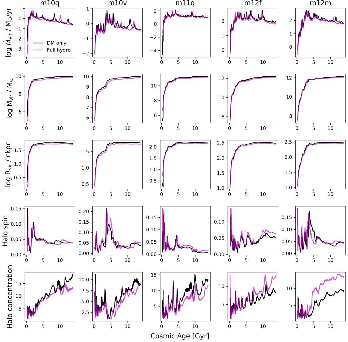
Figure 15. A few relevant halo properties measured in the full hydrodynamical simulations (magenta lines) and the corresponding DM-only simulations (black lines). These are the 5 halos for which corresponding DM-only FIRE-2 runs exist. The DM-only halo properties are very similar to the hydro-based halo properties, with the M_{\text{vir}} and R_{\text{vir}} being lower in the hydro version by only 10-20% on average. The major systematic difference is in the halo concentration which tends to be lower in the dwarfs in the hydro version (presumably due to stellar feedback adiabatically expanding the halo center) whereas it is higher for the MW-mass halos in the hydro run (presumably due to the significant stellar mass adiabatically contracting the halo center).
