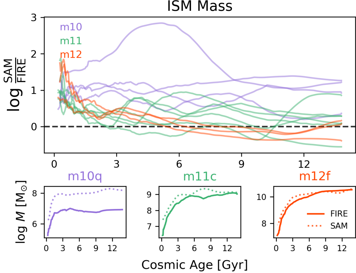
Figure 5. Similar to Figure 3 but now for ISM mass as a function of cosmic age. The SAM agrees relatively well with FIRE-2 for the m12 halos except at very early times, and this is also true for the m11 halos, albeit with more scatter. But the systematic discrepancy for the m10 halos remains at the order of magnitude level at all times, consistent with the z = 0 SAM excess in Figure 2.
