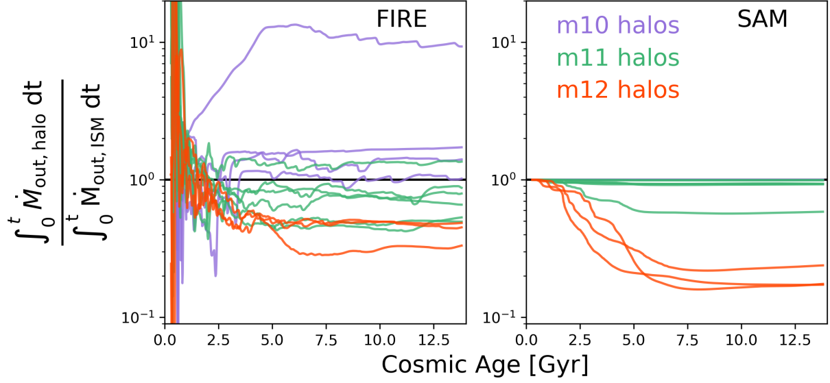
Figure 12. The ratio of the cumulative mass ejected from the halo versus from the ISM as a function of cosmic time for FIRE-2 (left panel) and the SAM (right panel). The lines are color-coded according to z = 0 halo mass. The SAM qualitatively follows the FIRE-2 trends for the m11 and m12 halos at z \lesssim 2 (i.e., cosmic ages \gtrsim 3 Gyr): an increasingly larger fraction of winds are able to leave the halo in progressively lower mass halos. But in the FIRE-2 simulations, the m10 halos strikingly tend to have expelled more material through R_{\text{vir}} than has ever left the ISM boundary ( 0.1R_{\text{vir}} ), implying significant entrainment of ambient CGM material by the outflows (this is also true for the progenitors of all halos at very early times z \gtrsim 6 ). Since the ratio cannot exceed 1 in the SAM by construction, it asymptotes to 1 for the low-mass dwarfs (all of their winds leave the halo).
