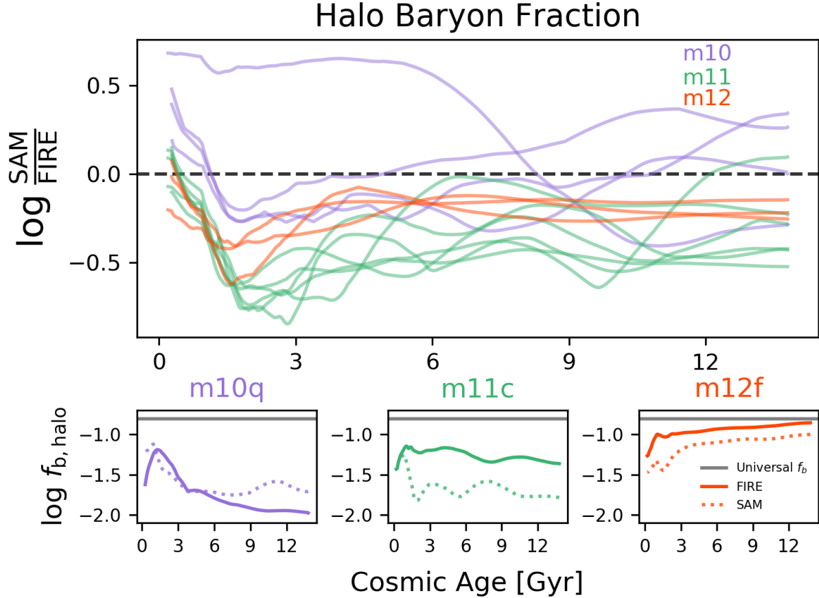
Figure 7. Similar to Figure 3 but now for the bulk halo baryon fractions. The SAM reproduces the general trend in FIRE-2: lower mass halos are more depleted of baryons than higher mass halos, relative to the universal baryon fraction (horizontal gray lines in the bottom panels; f_b = 0.158 according to Planck Collaboration et al. 2016). There is relatively good agreement between the SAM and FIRE-2, with differences at the factor of \sim 2 - 3 level at most (despite order of magnitude differences in ISM and CGM mass; note the much smaller y-axis range in this figure compared to Figure 5 and Figure 6).
