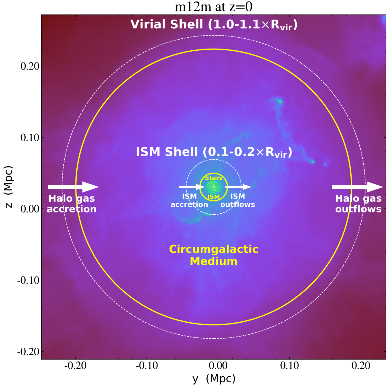
Figure 1. An illustration of our zone definitions for analyzing bulk and flow quantities in the FIRE-2 simulations. The background image shows the projected gas density distribution of the MW-mass halo m12m at z = 0 (purple is low density, with green and yellow representing progressively higher densities, respectively). The solid yellow circles represent the virial radius (outer circle) and the “edge” of the ISM (inner circle). The dashed white circles demarcate the outer limits of the virial and ISM shells ( 1.0 - 1.1 \times R_{\text{vir}} and 0.1 - 0.2 \times R_{\text{vir}} , respectively) through which mass inflow and outflow rates are computed. Stellar and ISM masses are computed using all star and gas particles within 0.1 \times R_{\text{vir}} , respectively, whereas CGM masses are computed using all gas particles between 0.1 - 1.0 \times R_{\text{vir}} . These definitions are well-matched for comparison to the Santa Cruz SAM.
