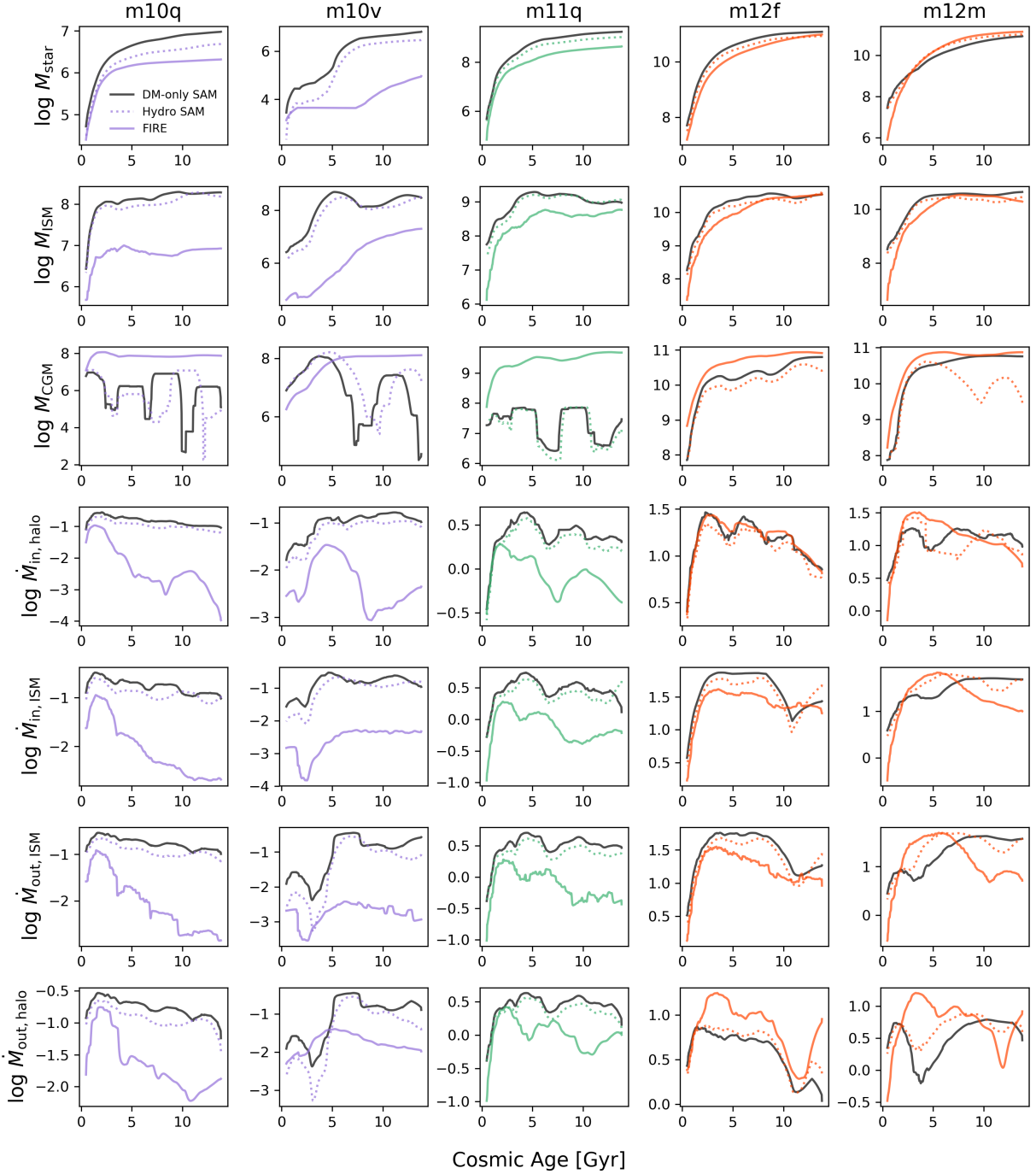
Figure 16. Time series of the main properties considered in the paper for the five individual halos with corresponding DM-only simulations. From left to right: m10q, m10v, m11q, m12f and m12m. From top to bottom: stellar mass, ISM mass, CGM mass, halo gas mass inflow rate, ISM mass inflow rate, ISM mass outflow rate and halo mass outflow rate. In every panel, the solid black line shows the prediction of the SAM when run on the DM-only simulation merger trees. The other two curves follow the same convention as the individual halo panels in the figures from the main body of the paper: solid colored curves for the FIRE-2 measurements and dotted colored curves for the SAM predictions using the full hydrodynamical simulation merger trees. The colors show the mass bin that each halo belongs to (purple for m10, green for m11 and red for m12). The main takeaway is that our conclusions do not change if we use the SAM results from the DM-only simulation merger trees: the new SAM predictions agree with our fiducial ones relatively well, and hence the DM-only-based SAM trends relative to FIRE-2 remain qualitatively the same.
