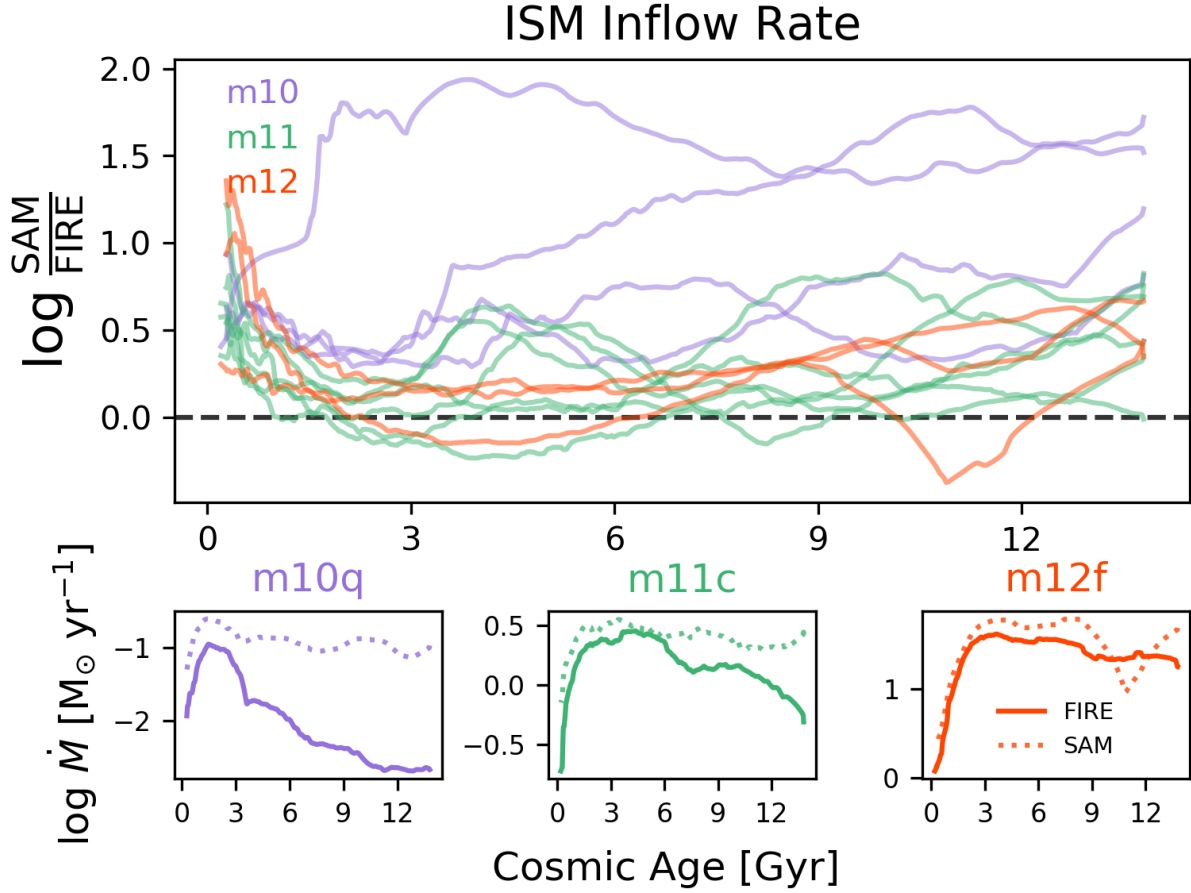
Figure 9. Similar to Figure 3 but now for ISM gas accretion rate. The SAM generally has higher ISM gas accretion rates than measured in FIRE-2, and this discrepancy is preferentially worse for the lower mass halos (up to two orders of magnitude). Even the m12 halos at late times have about a factor of two higher ISM accretion rates in the SAM than in FIRE-2.
