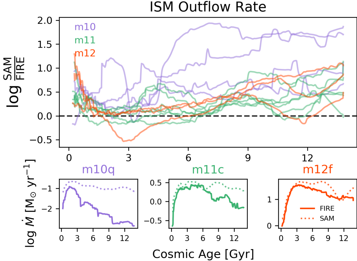
Figure 10. Similar to Figure 3 but now for the ISM mass outflow rate. The SAM has higher ISM outflow rates than FIRE-2, with the discrepancy becoming larger than a factor of two for most halos by late times. This is necessary in the SAM to prevent excess star formation and match the observed stellar mass function.
