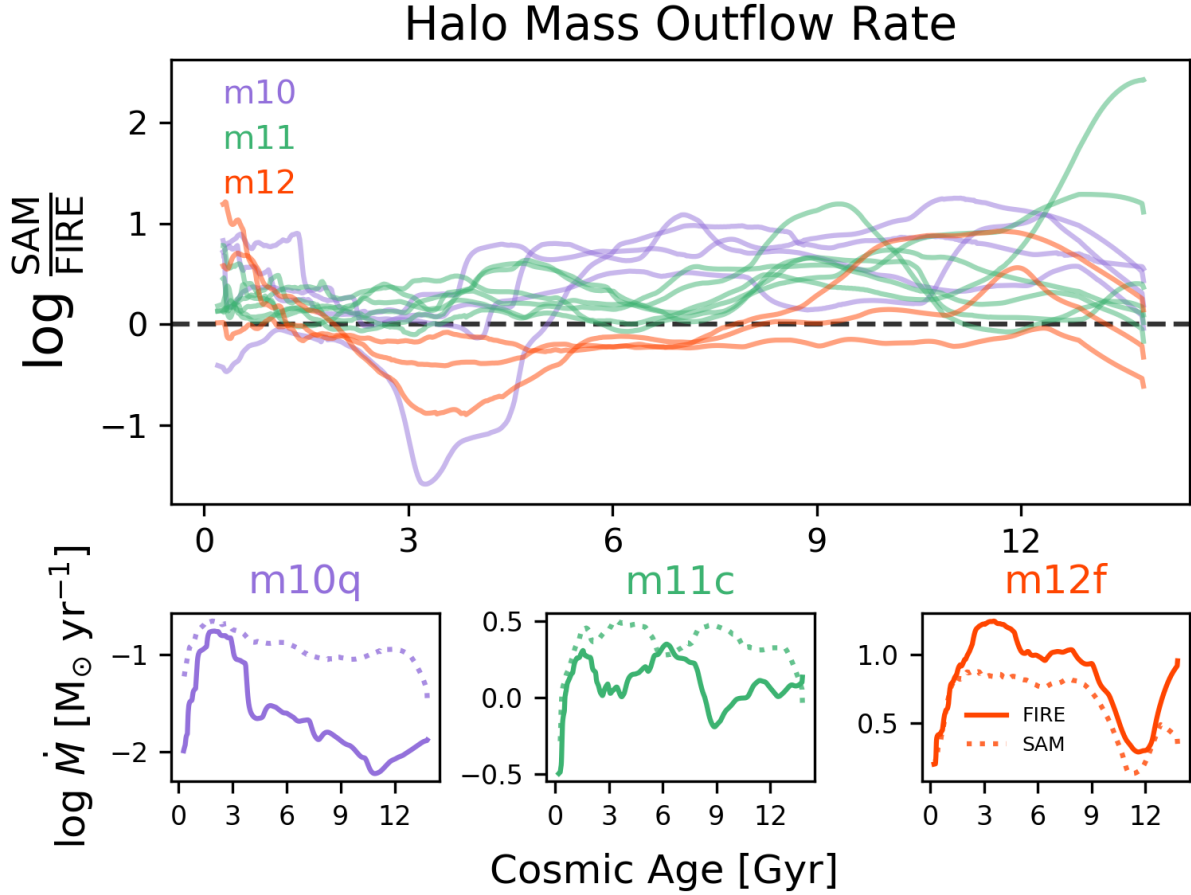
Figure 11. Similar to Figure 3 but now for the halo mass outflow rates. The SAM has higher halo mass outflow rates than the FIRE-2 measurements. This is not surprising because the halo mass outflow rate in the SAM is a halo circular velocity-dependent re-scaling of the ISM outflow rate, and the latter was already shown to be much higher than FIRE-2.
